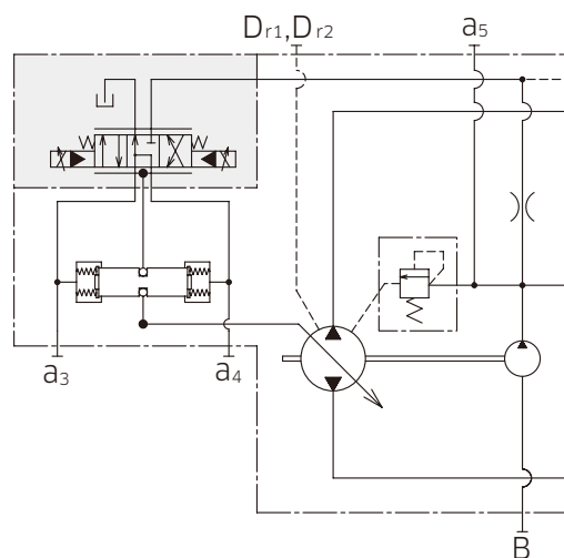
Hydraulic circuit
