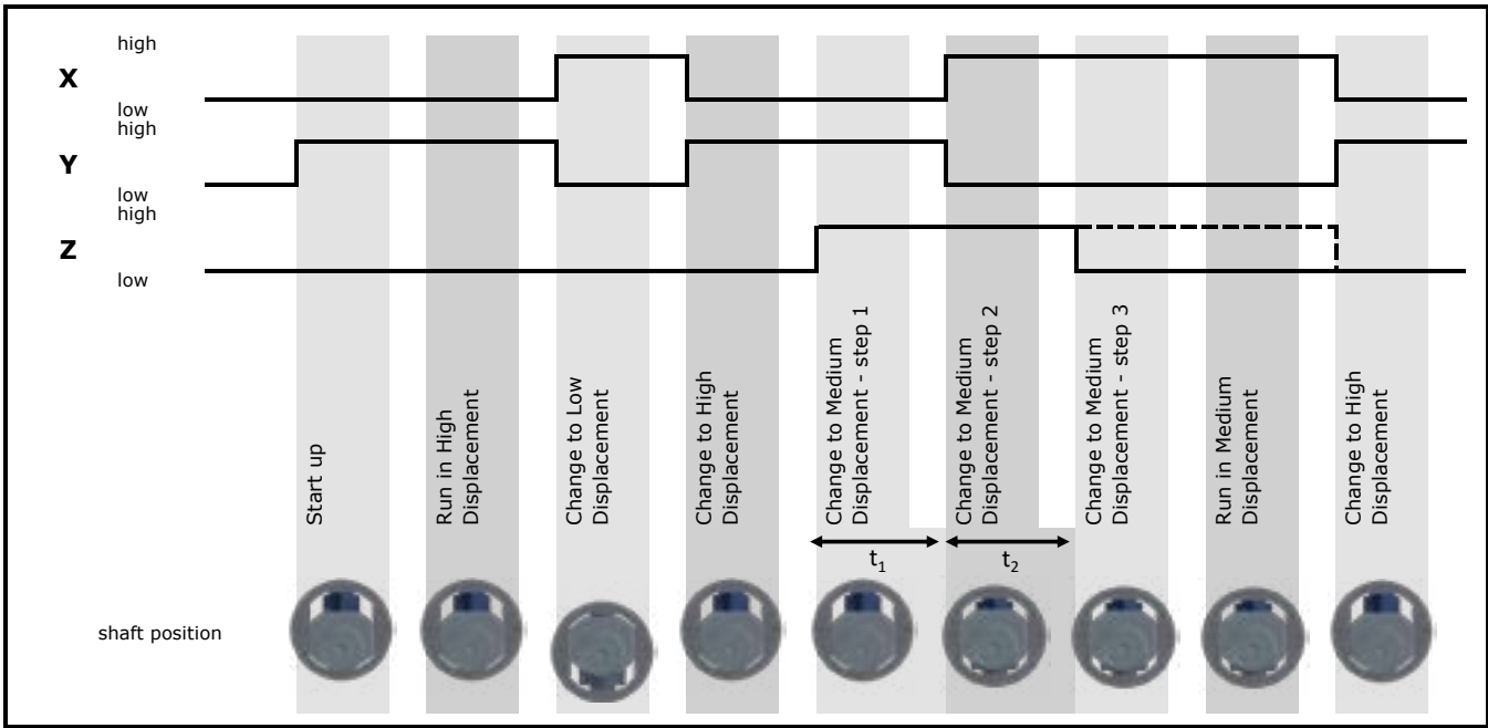
◆ Displacement Sequence Control Timing
