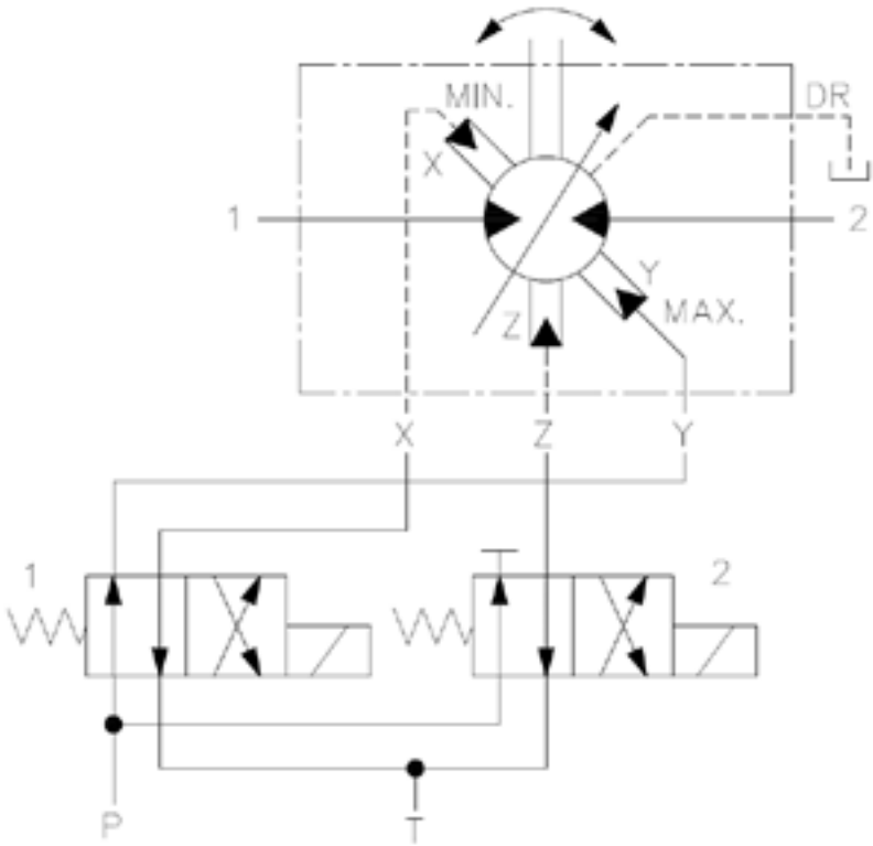
◆ Displacement Sequence Control Schematic
