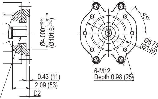
SAE B 30° Involute Spline SAE J744-22-4 13T 16/32DP
