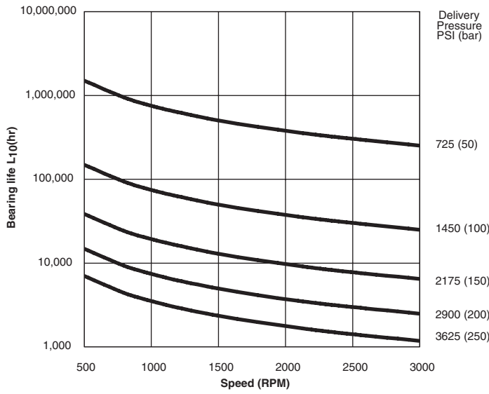
Bearing Life
