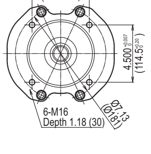
SAE C 4 hole 4.500 +0.007 (114.5 +0.20 )
