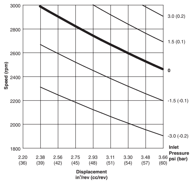
Self-priming Capability
