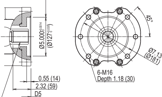
SAE CC 30° Involute Spline SAE J744-38-4 17T 12/24DP
